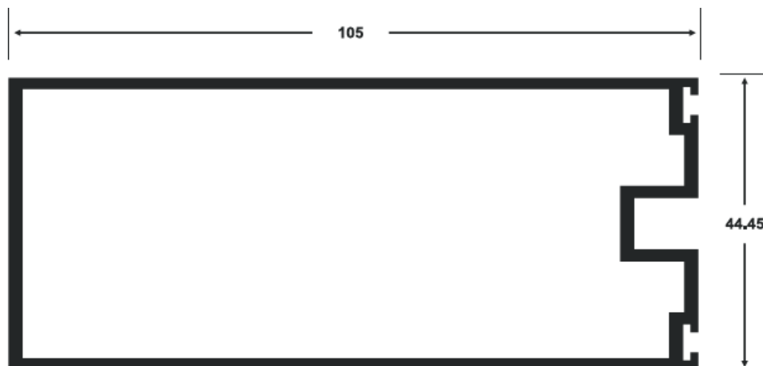
4501 Mullion
