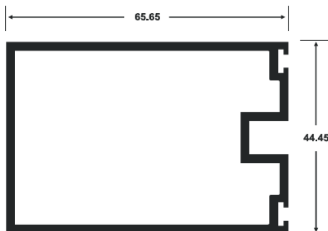
4502 Mullion
